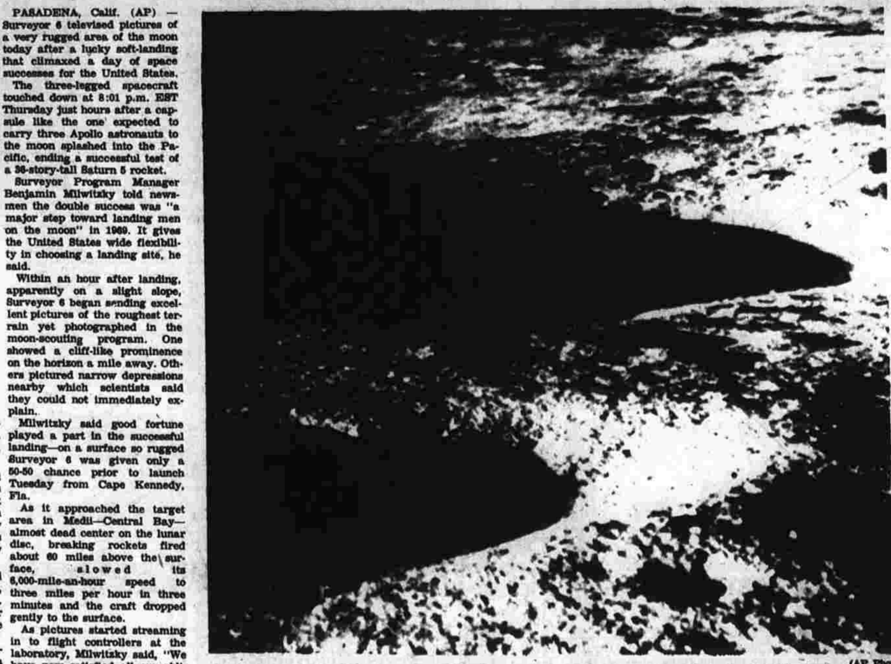
Long dark craters dominate this picture of the Moon taken today by America's Surveyor 6. The general scene is a large crater, with horizon at top of picture several hundred yards from the space-craft camera. Pictures made looking south, about three hours after spacecraft landing.
